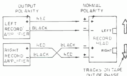
Figure 4. Leads can be placed incorrectly on the recording head and cause phasing problems in stereo recorders.
